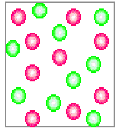
PLASMA
