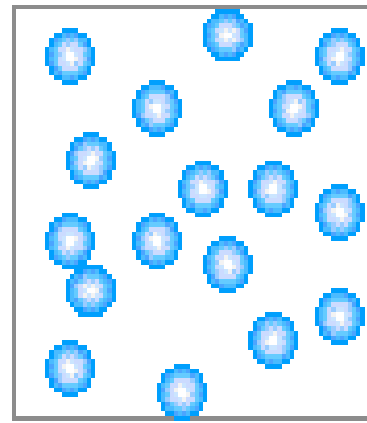
GAS
