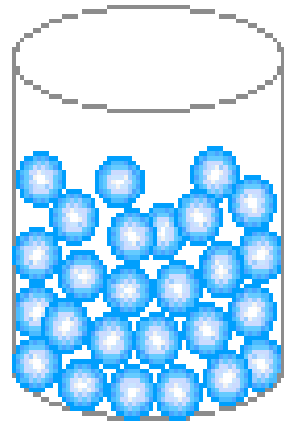
LIQUID
