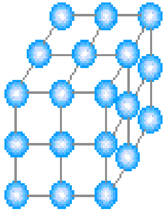
SOLID
